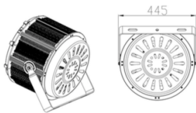
Fig. 1 Base view
